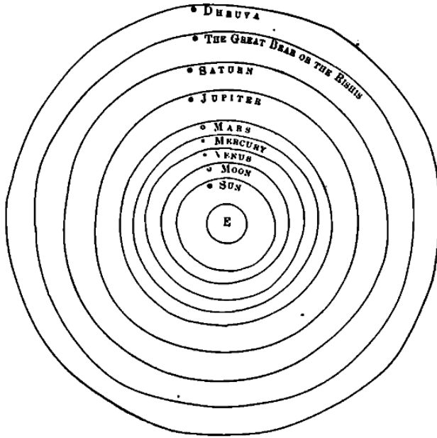
Positions of the planets.
