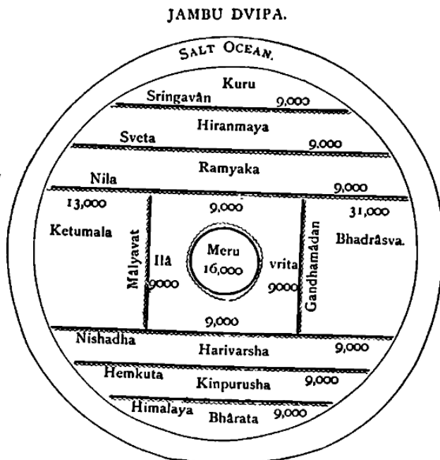
A diagram of Jambu-Dvīpa.
