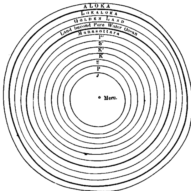
A diagram of the Bhûr system.
